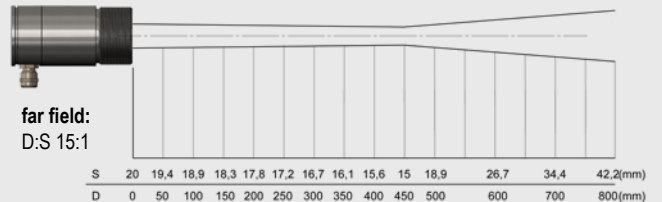
CF4 - optics 30:1 15 mm @ 450 mm
