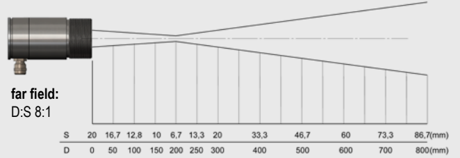
CF3 - optics 30:1 6.7 mm @ 200 mm
