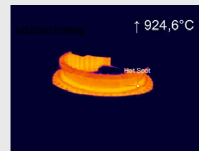
Induction heating
