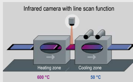
Glass tempering: Small optris IR cameras replace old bulky mechanical scanners
