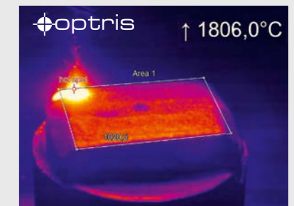
Measurement during laser welding process
