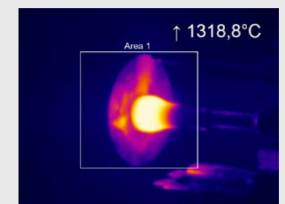
Electrical upsetting
